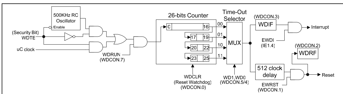
Figure 15-1: Watchdog Timer
