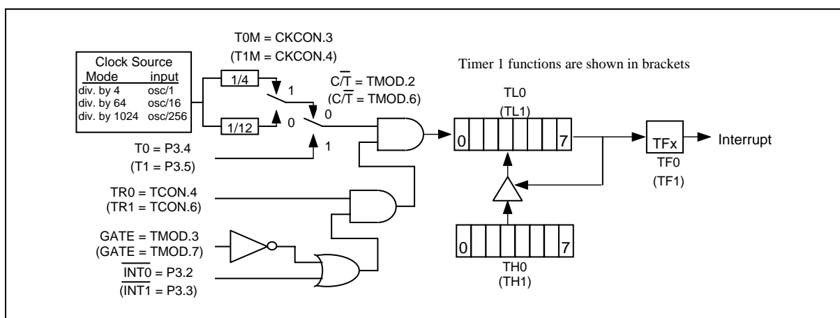
Figure 12. Timer/Counter Mode 2.
