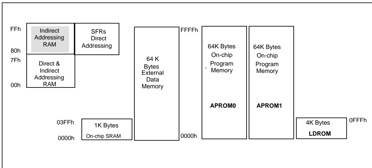
Figure 1. Memory Map
