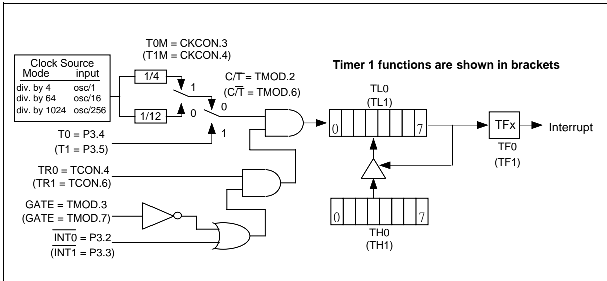
Figure 12: Timer/Counter Mode 2
