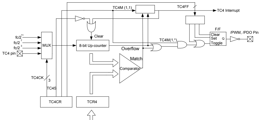
Fig. 25. Timer/Counter 4 Configuration
