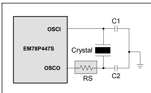
Fig. 4-10 Crystal/Resonator Circuit
