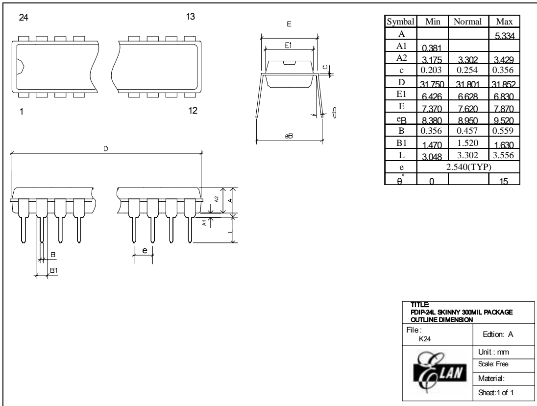
24-Lead Plastic Dual Inline Skinny Package ( SDIP ) - 300 mil
