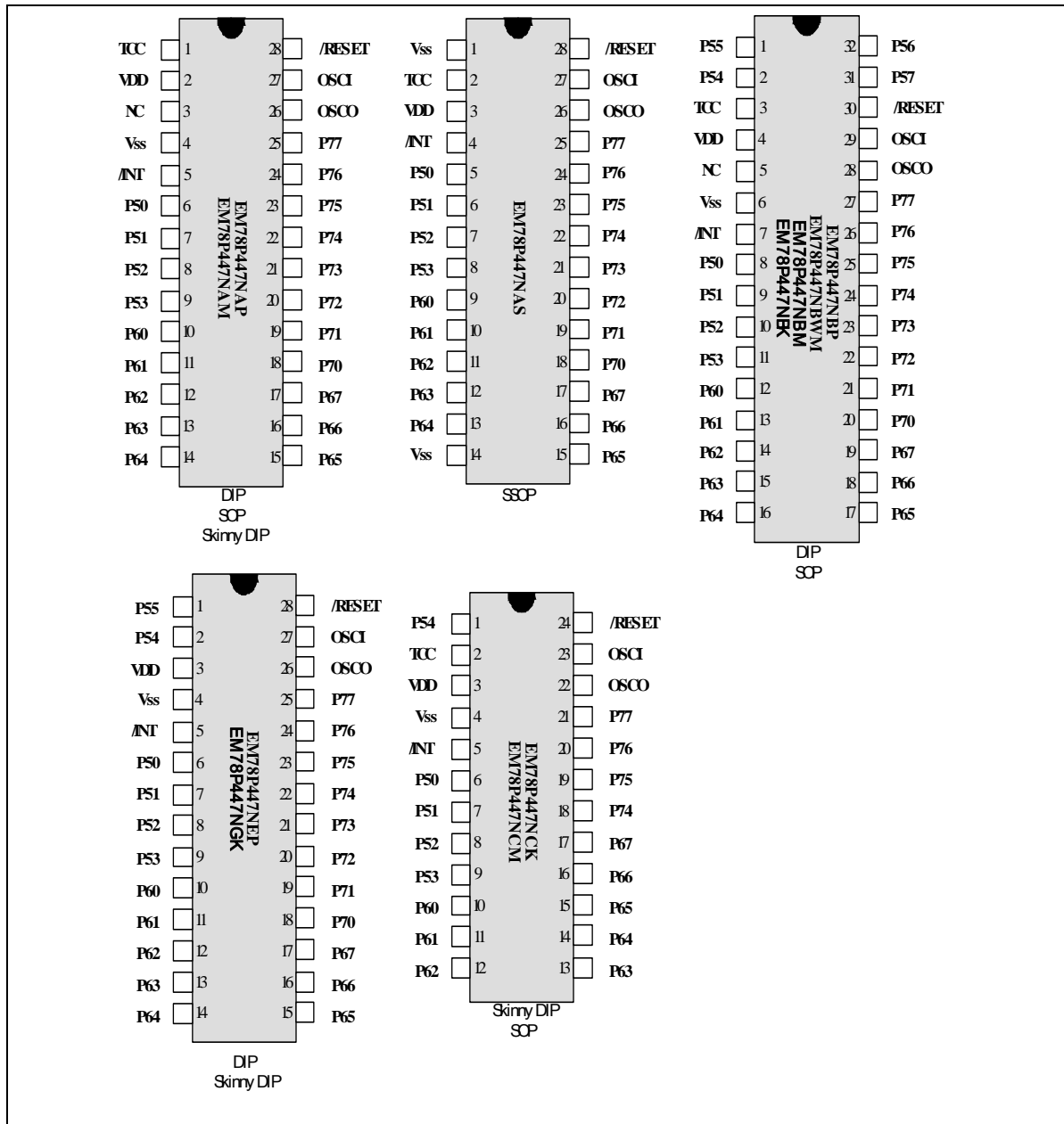
Fig. 3-1 Pin Assignment
