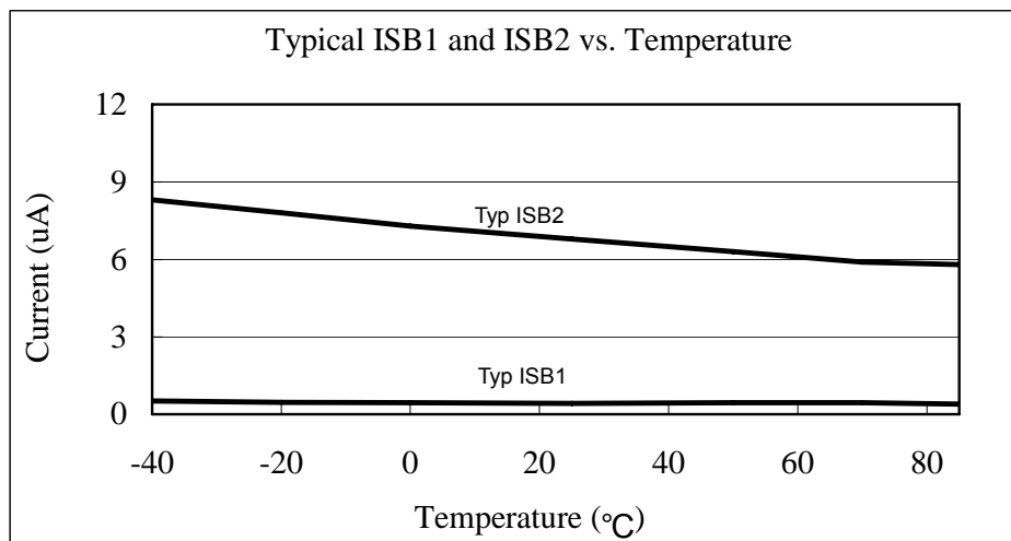
Fig. 6-16 Typical Standby Current ( ISB1 and ISB2 ) vs. Temperature
