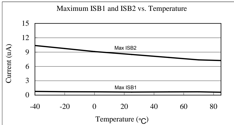
Fig. 6-17 Maximum Standby Current ( ISB1 and ISB2 ) vs. Temperature
