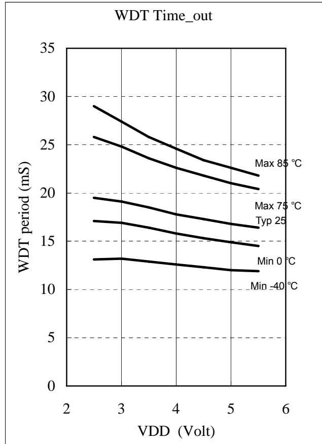
Fig. 6-9 WDT Time Out Period vs. VDD, Prescaler Set to 1 : 1
