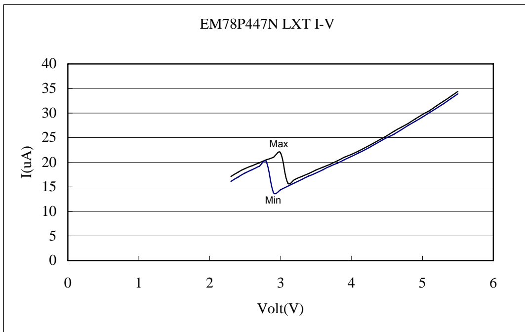
Fig. 6-20 EM78P447N I-V Curve Operating at 32.768 kHz
