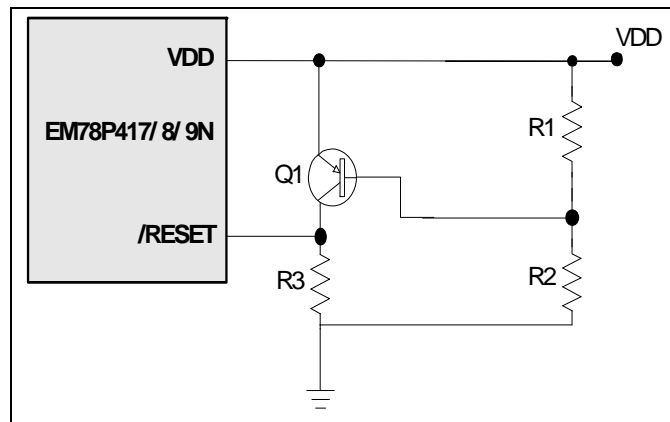
Fig 6-20 Residual Voltage Protection Circuit 2
