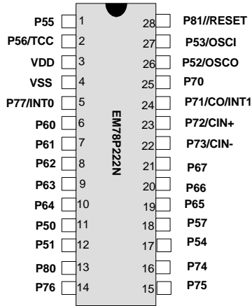
Fig. 3-1 EM78P222NK/AK/M/AM Pin Assignment
