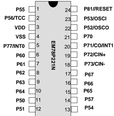
Fig. 3-2 EM78P221NK/M/AM Pin Assignment
