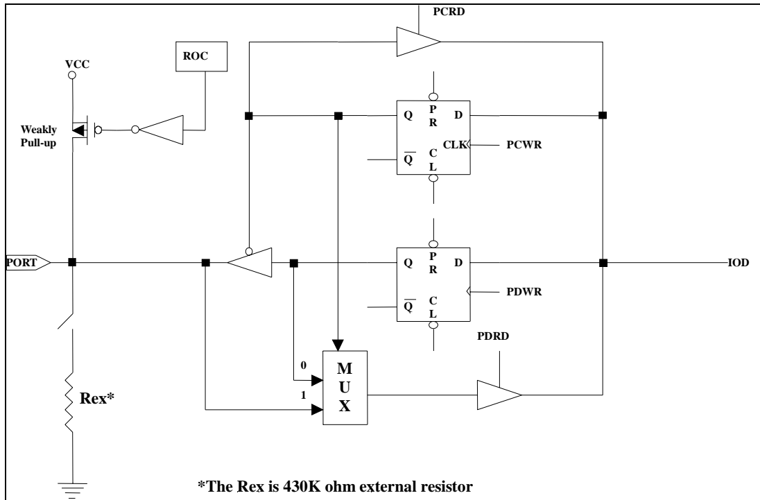
Figure 5-5 I/O Port with R-option (P50,P51) Circuit
