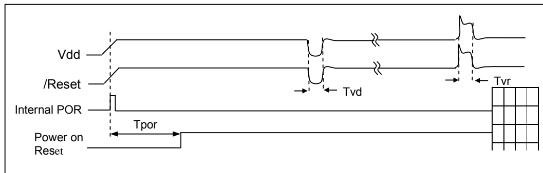
Figure C-1 EM78P154N Power-On Reset and Vdd Voltage Drop/Rise Timing Test Timing Diagram
