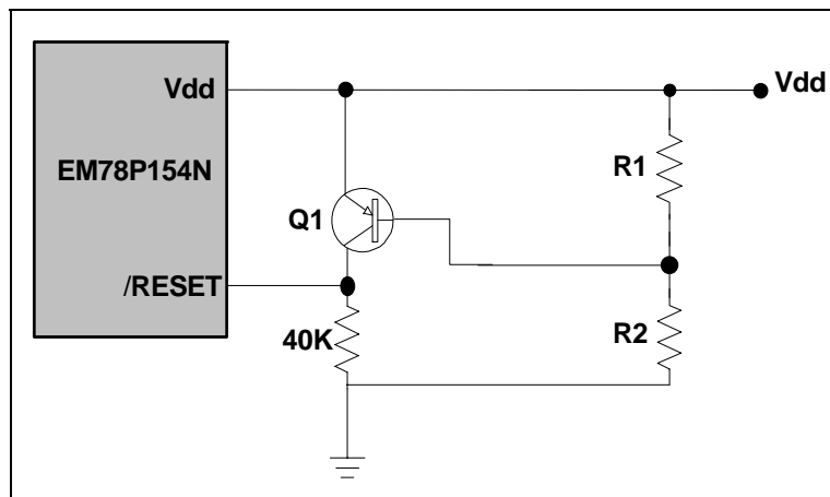
Figure 5-11b Residue Voltage Protection Circuit (2)
