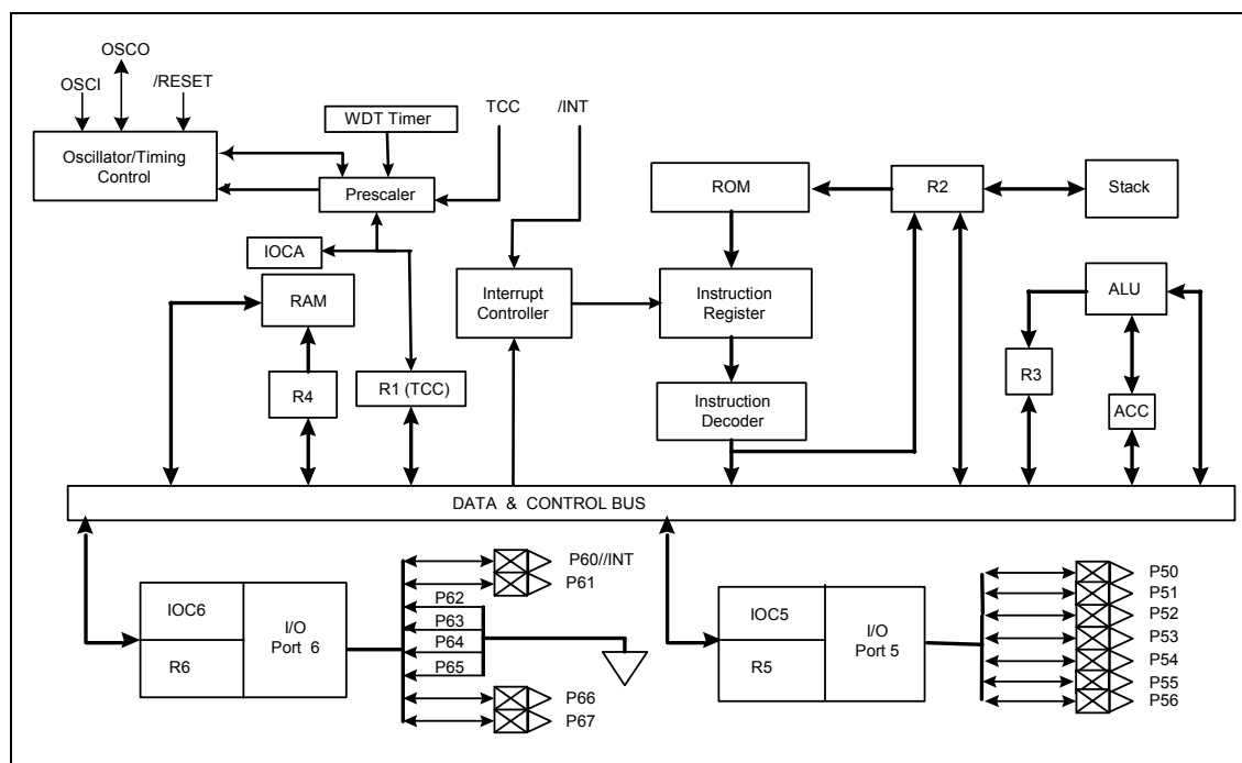
Figure 5-1 Function Block Diagram
