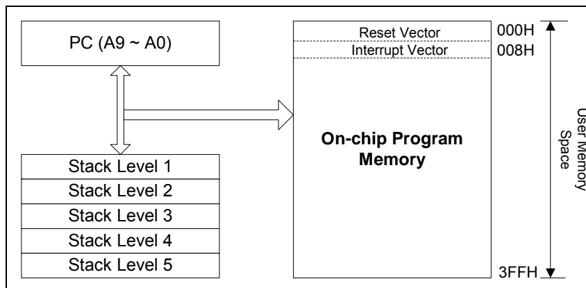
Figure 5-2 Program Counter Organization
