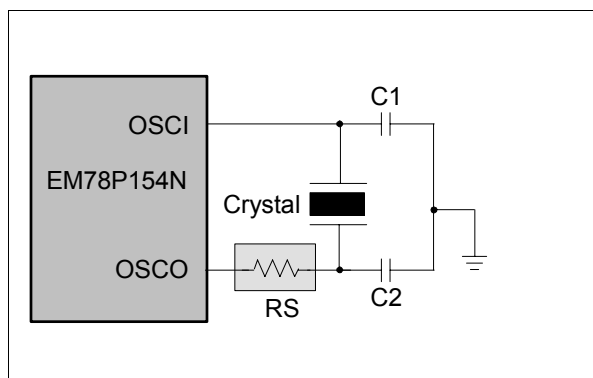
Figure 5-8b Crystal/Resonator Circuit
