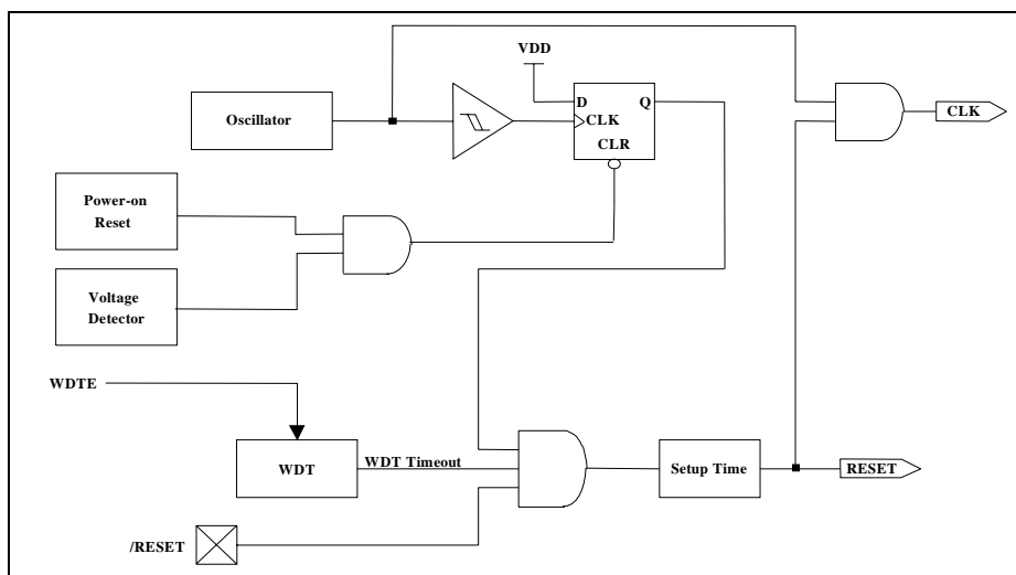
Figure 5-6 Controller Reset Block Diagram
