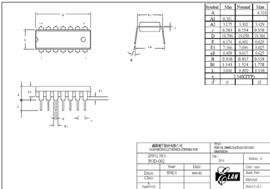
Figure B-1a EM78P154N 14-Lead PDIP Package Type
