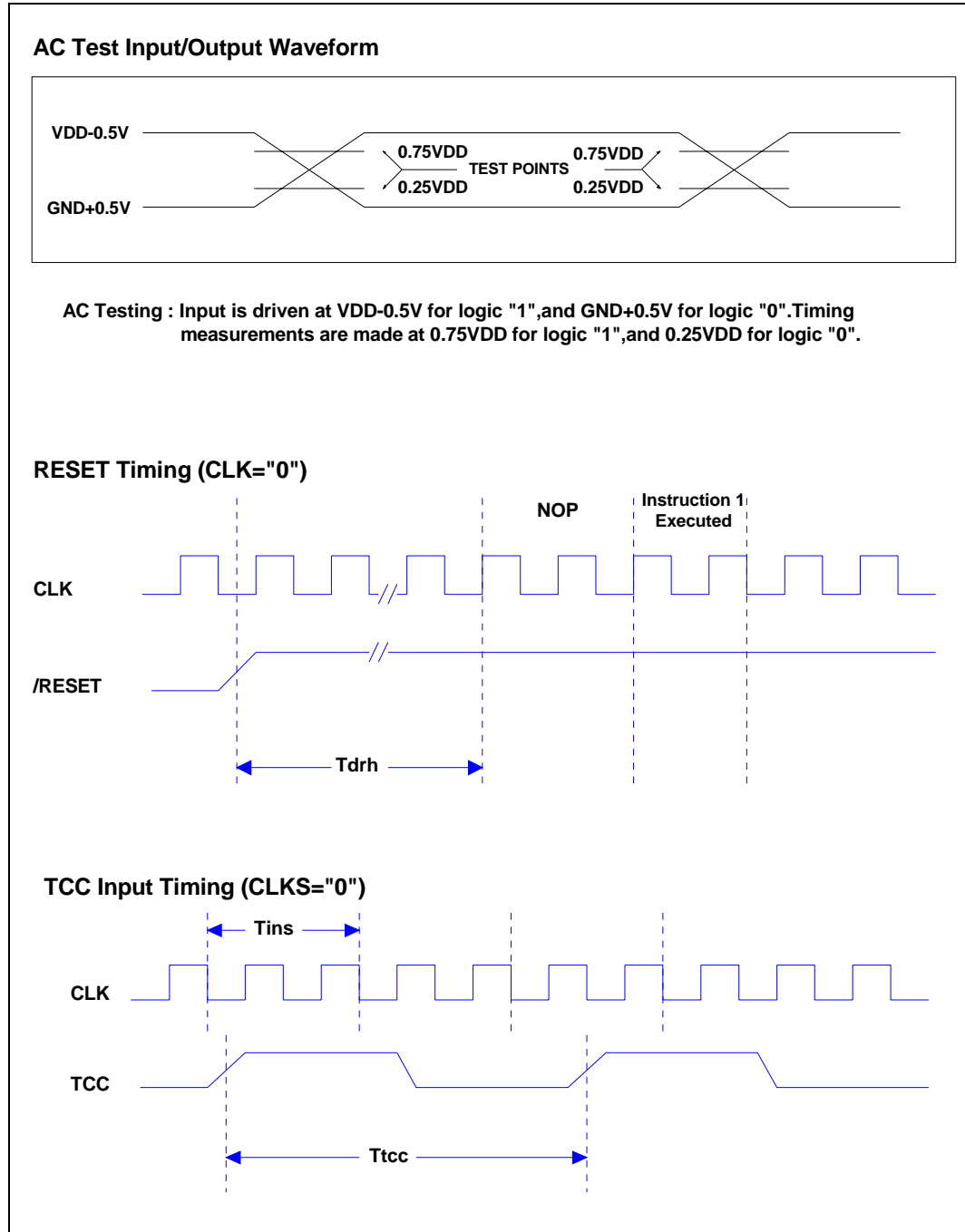
Figure 5-12 EM78P154N Timing Diagrams
