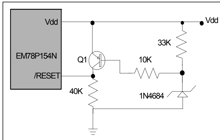
Figure 5-11a Residue Voltage Protection Circuit (1)
