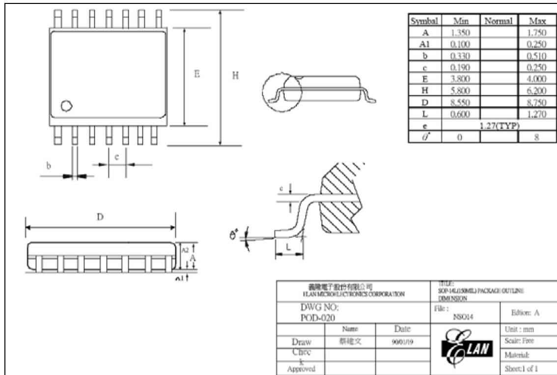
Figure B-1b EM78P154N 14-Lead SOP Package Type
