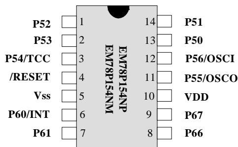
Figure 3-1a EM78P154NP/M Pin Assignment
