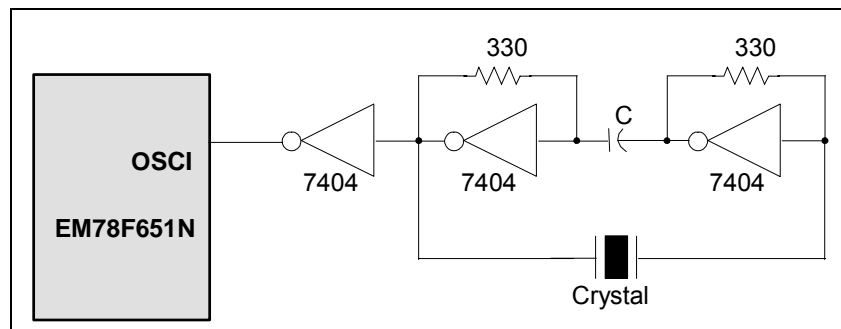
Fig. 6-12 Circuit for Crystal/Resonator-Series Mode
