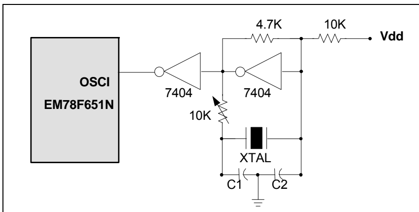
Fig. 6-13 Circuit for Crystal/Resonator-Parallel Mode
