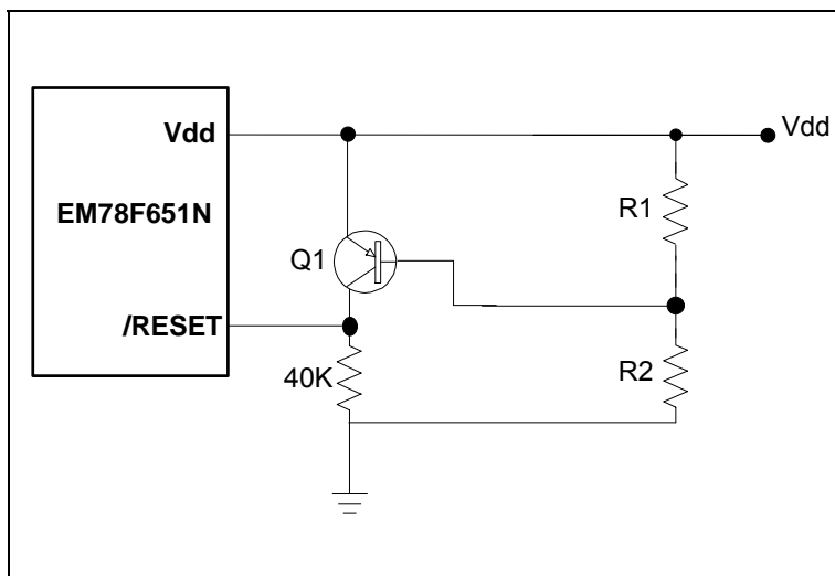
Fig. 6-17 Circuit 2 for the Residue Voltage Protection
