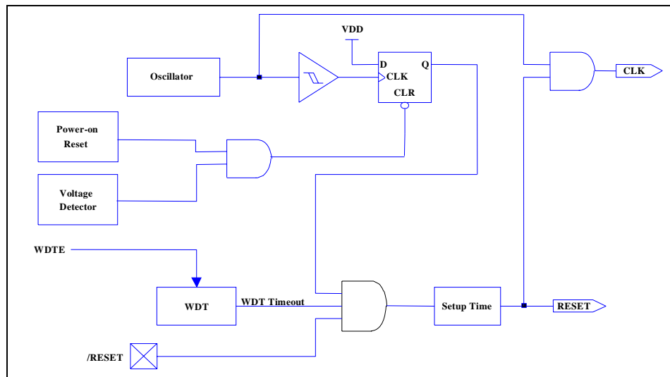
Fig. 6-6 Block Diagram of Controller Reset
