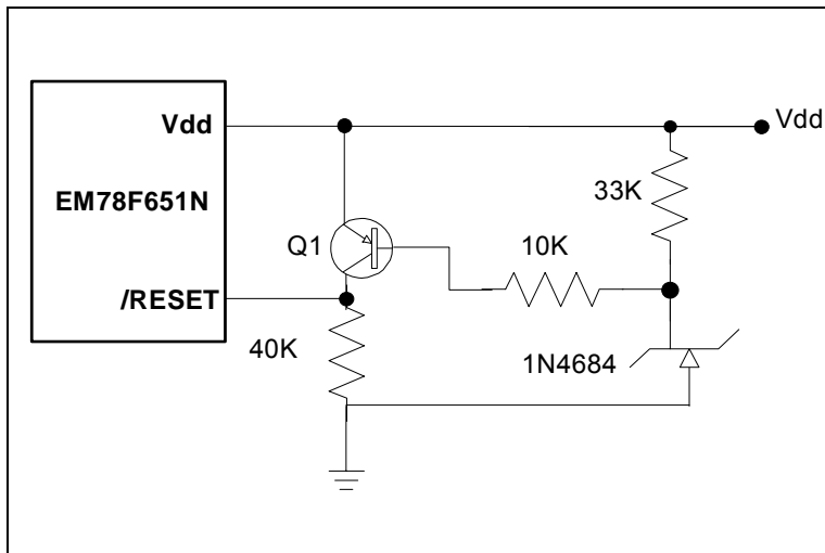
Fig. 6-16 Circuit 1 for the Residue Voltage Protection
