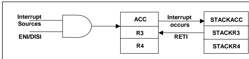
Fig. 6-8 Interrupt Back-up Diagram
