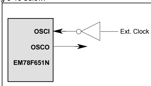
Fig. 6-10 Circuit for External Clock Input
