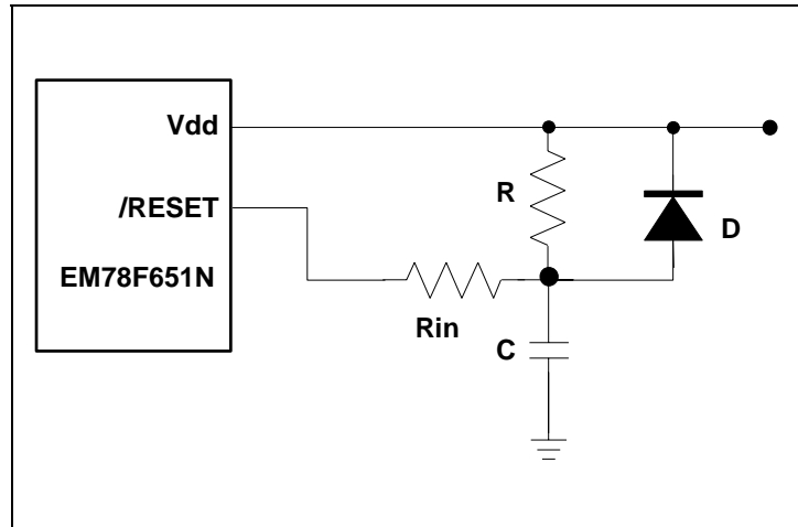
Fig. 6-15 External Power-Up Reset Circuit
