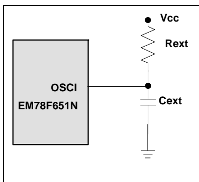
Fig. 6-14 Circuit for External RC Oscillator Mode
