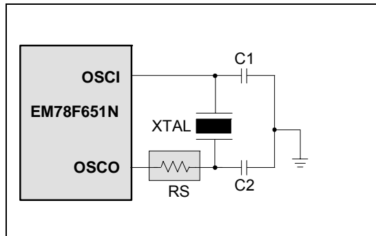
Fig. 6-11 Circuit for Crystal/Resonator
