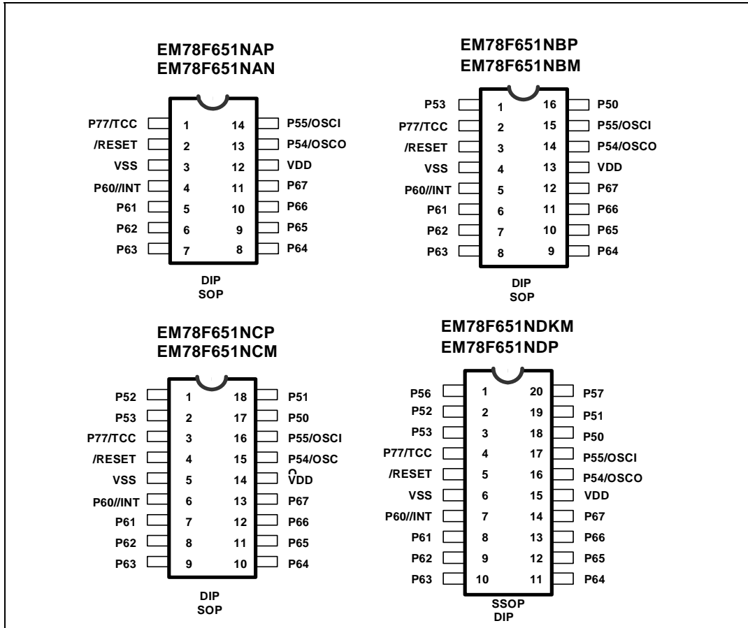
Fig. 3-1 Pin Assignment
